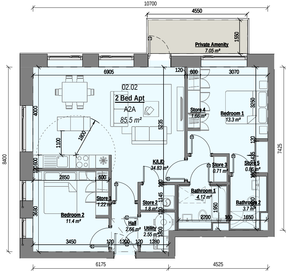
1 APARTMENT TYPE A2A Scale: 1 : 100
