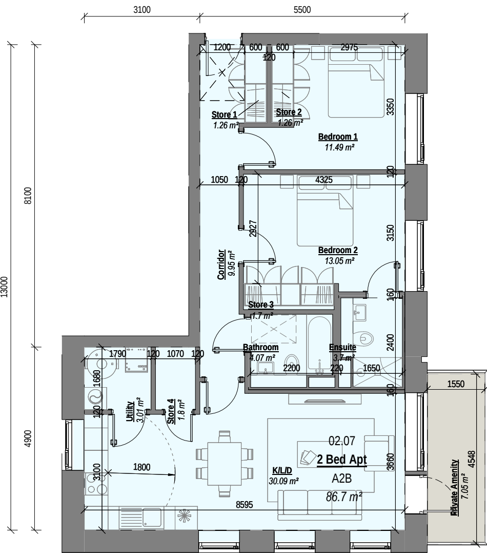
1 APARTMENT TYPE A2B Scale: 1 : 100
