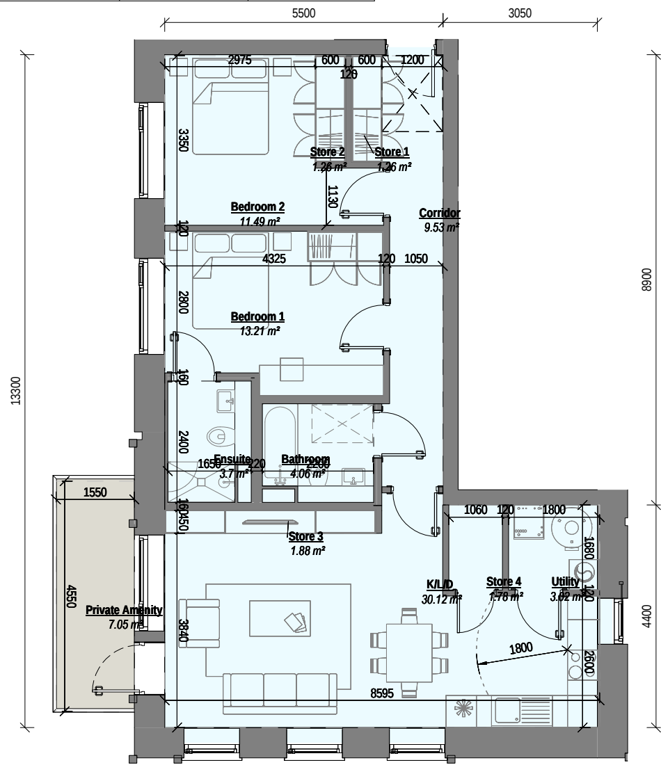
1 APARTMENT TYPE A2C Scale: 1 : 100
