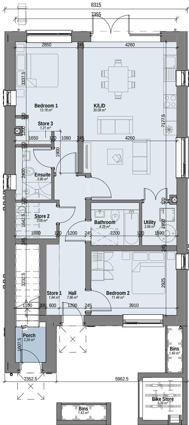
1 DAD - Level 00 Scale: 1 : 100
