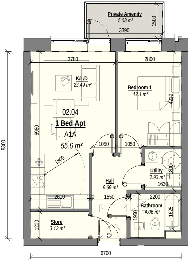
1 APARTMENT TYPE A1A Scale: 1 : 100
